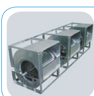
CBP-TE Double inlet triplex centrifugal fans
